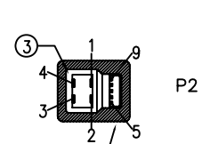
USB3.0 B TYPE MALE
