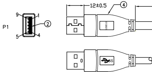
USB3.0 A TYPE MALE
