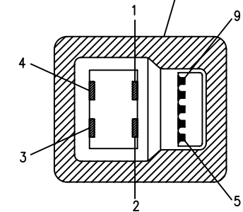
USB 3.0 B M-PIN SPEC.
