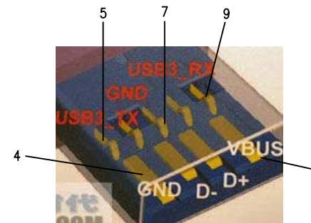
USB 3.0 A M-PIN 3D SPEC.
